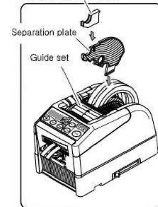
Auxiliary separation plate
